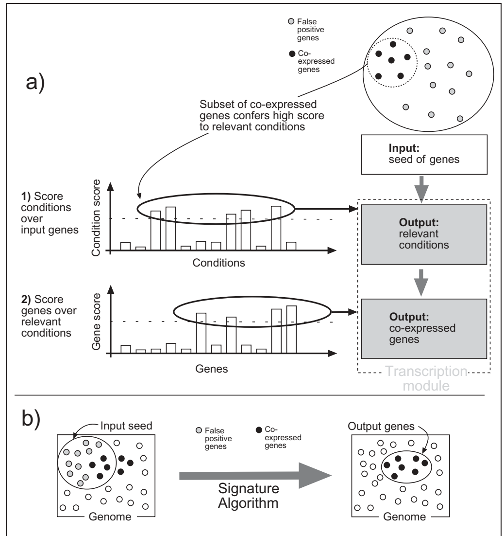
Figure 2: The Signature Algorithm requires as input a set of genes, some of which are expected to be co-regulated based on additional biological information such as a common promoter binding motifs or functional annotation. (a) The algorithm proceeds in two steps: in the first step, this input seed is used to identify the conditions that induce the highest average expression change in the input genes. Only conditions with a score above some threshold are selected. In the second stage of the algorithm, genes that are highly and consistently expressed over these conditions are identified. The result consists of a set of co-regulated genes together with the regulating conditions and is termed a transcription module . (b) The output contains only the co-regulated part of the input seed, as well as other genes that were not part of the original input but display a similar expression profile over the relevant conditions
